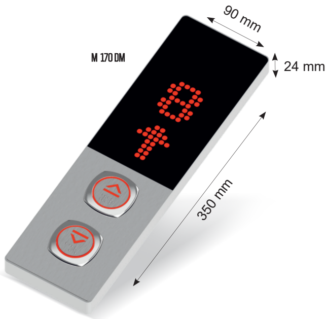
Kapak (Cover): 90*350*24mm
