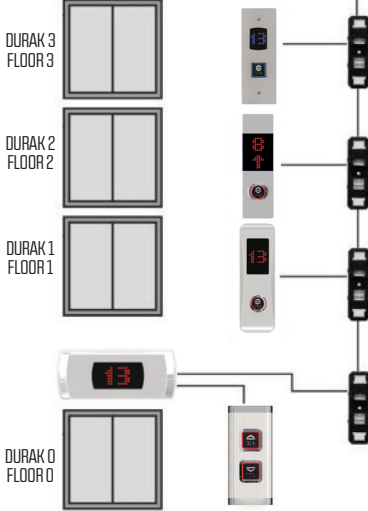
CAN BUS Kat Tesisi Can Bus Floor Installation
