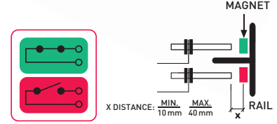
Positions of the contacts of the switch against magnet Mounting of the bi-stable switch on the cabin
