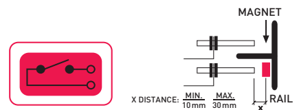
Positions of the contacts of the switch against magnet Mounting of the mono stable switch on the cabin
